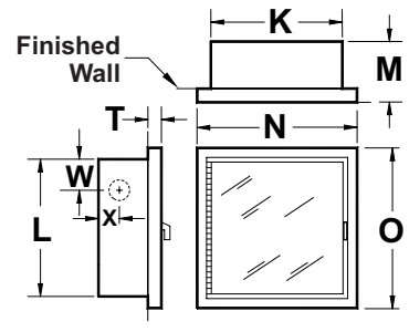
SEMI-RECESSED
