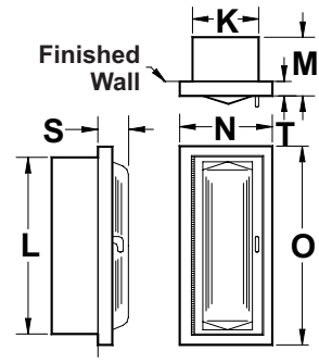
SEMI-RECESSED
