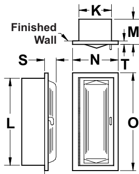
RECESSED
