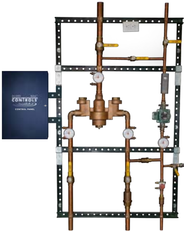
COMMAND STATION WITH BASyC ™ MODEL NO. CSMV SERIES
